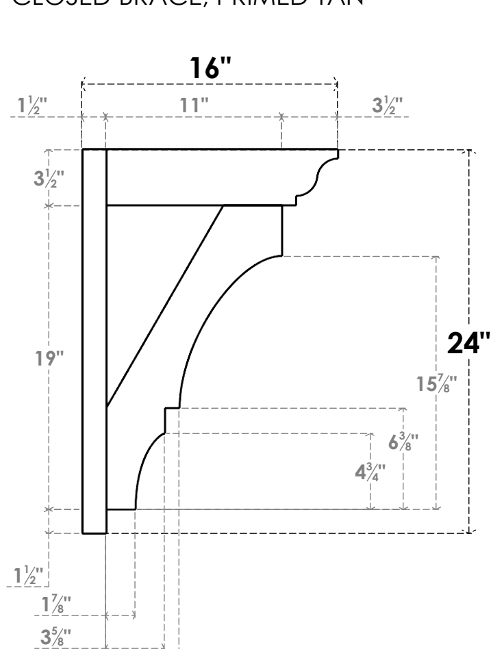
SIDE PROFILE
